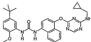
1-(5-tert-Butyl-2-methoxy-phenyl)-3-{4-[4-(cyclopropylmethyl-amino)-[1,3,5]triazin-2-yloxy]-naphthalen-1-yl}-urea;
